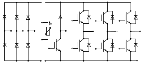
Internal Circuit
