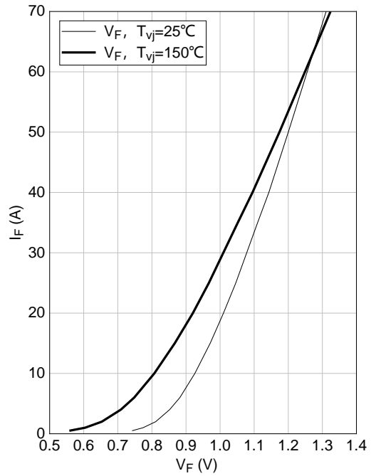
Forward characteristic of Diode, Rectifier (typical) I_F = f(V_F)
